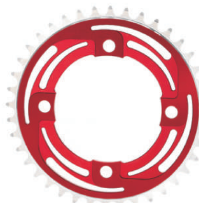
CC-CH 36T-53T THICKNESS 4mm BCD 104mm For Single speed
